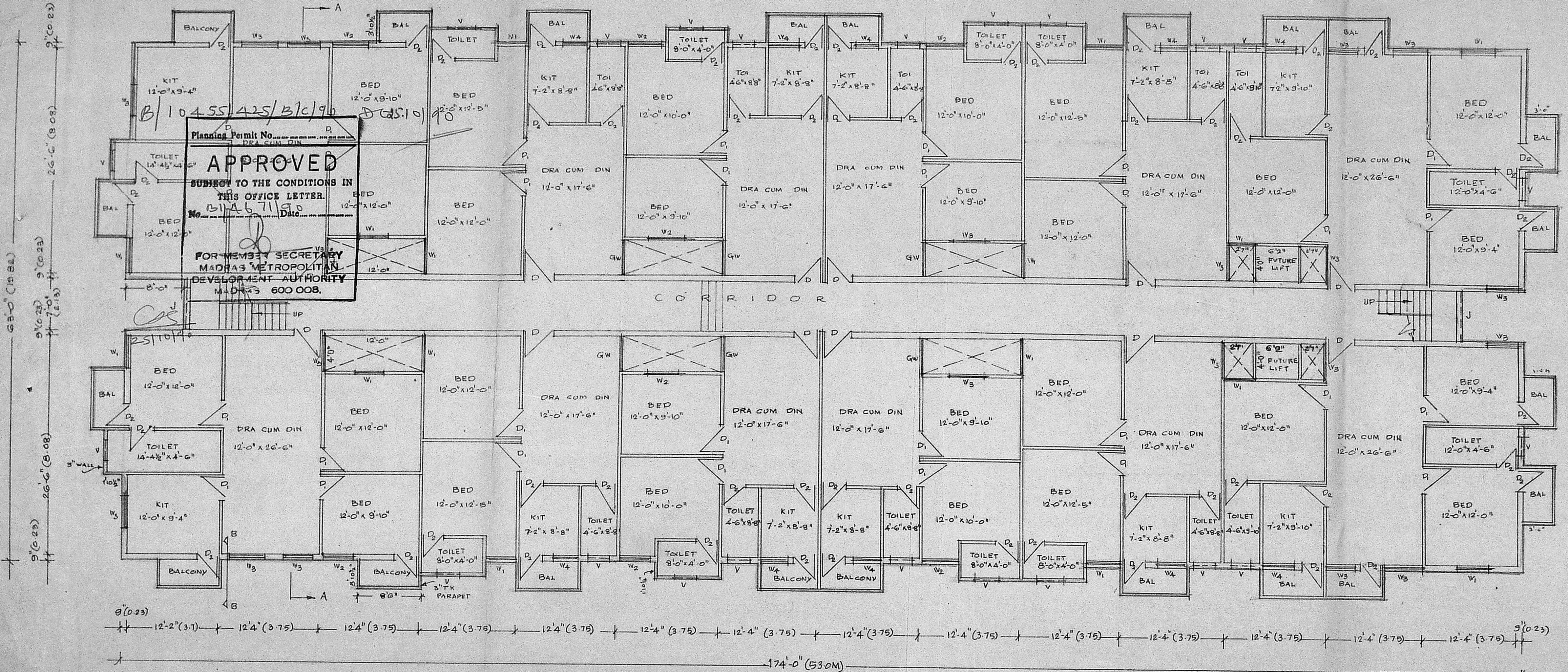
PLAN OF FIRST AND SECOND FLOOR
