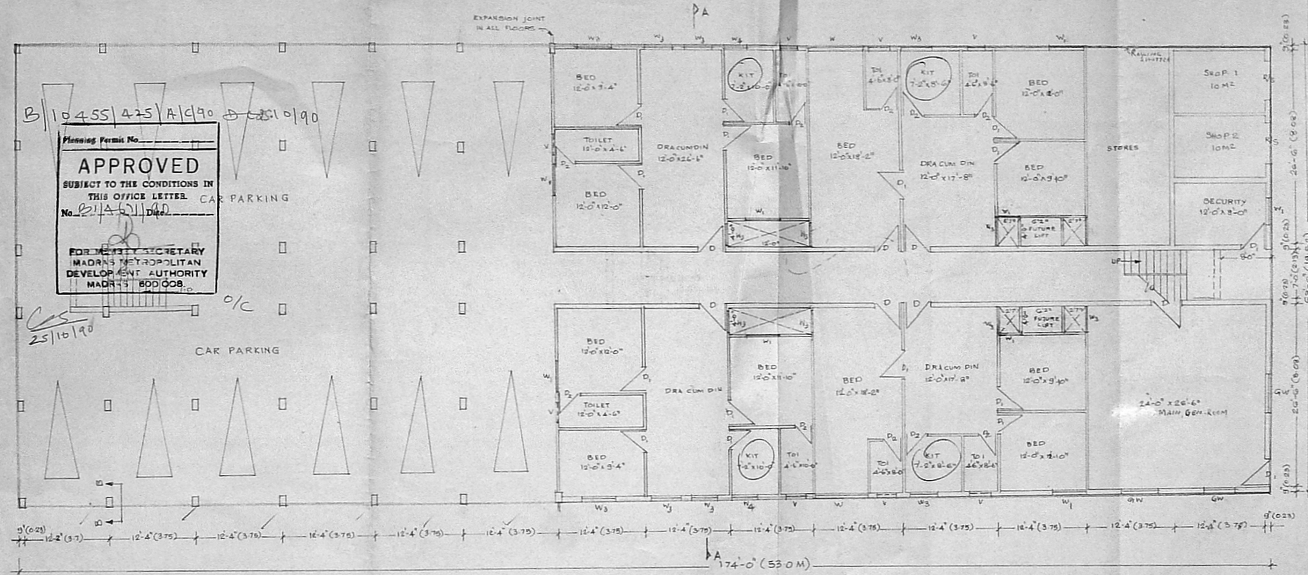
PLAN OF GROUND FLOOR
